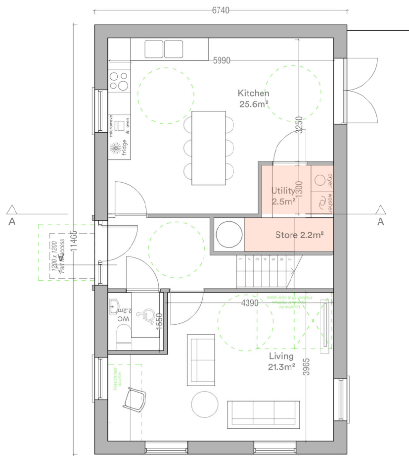
House Type U Ground Floor Plan 65.0 m 2
