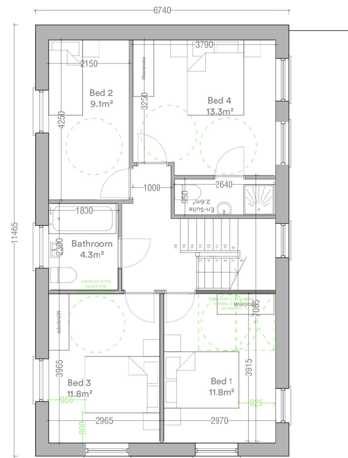
House Type U First Floor Plan 64.7m 2
